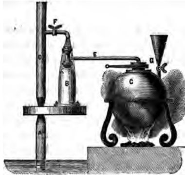
FIG. 12.—Savery's Engine, 1698.
